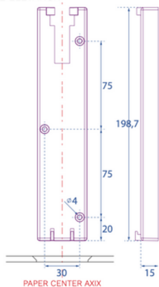
SIDE ELEVATION
